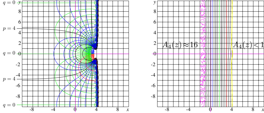
FIGURE 4. Left: Function f = F_{4,5}(z) in the x+iy plane; levels p = \Re(f)=\text{const} and levels q = \Im(f)=\text{const} are shown with thick lines for integer values of p and q . Right: Function f = A_4(z) by (4.13) in the x+iy plane; levels f = 1, 4, 8, 12, 16 are shown with thick lines.
